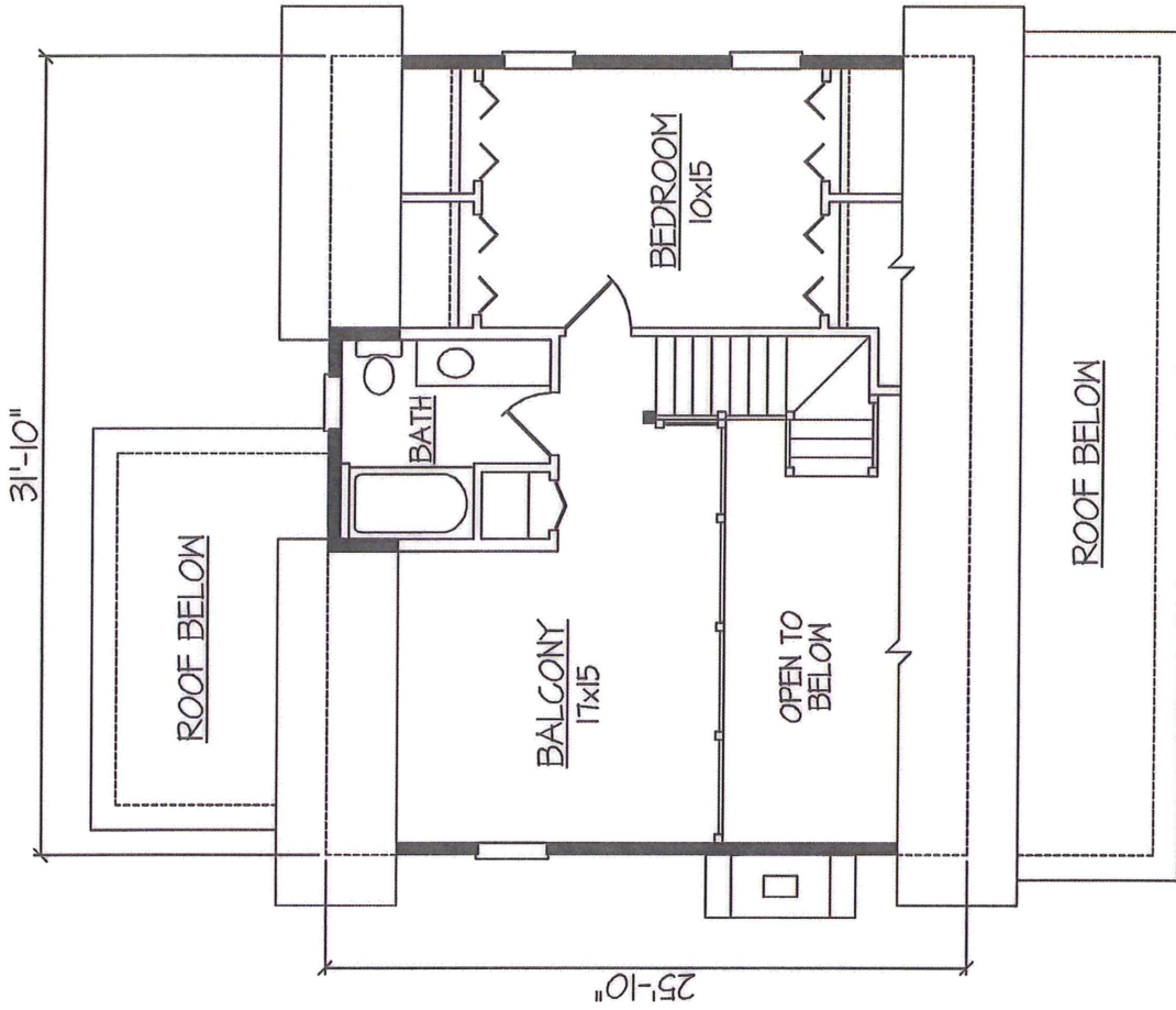
SECOND FLOOR PLAN SECOND FLOOR - 521 SF
