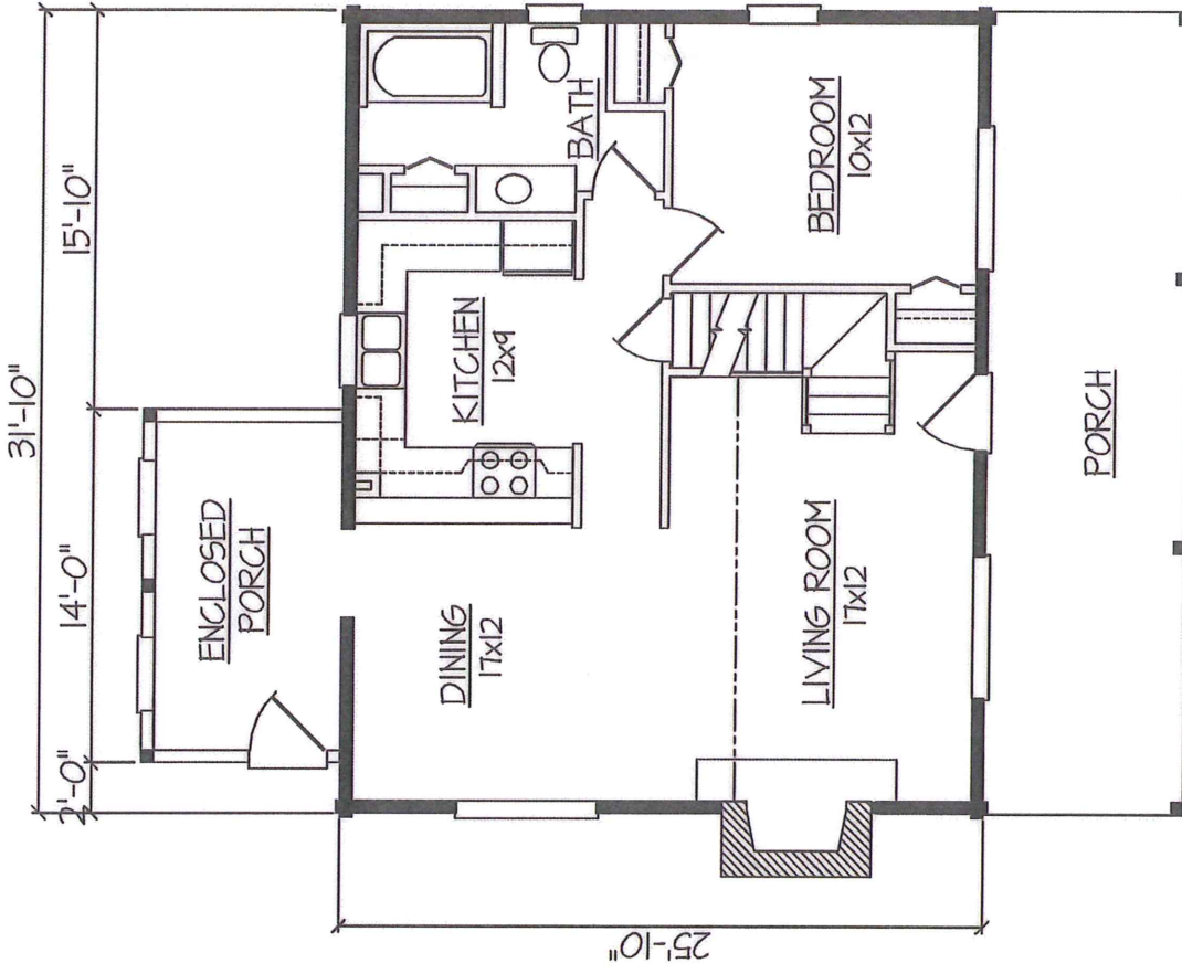
FIRST FLOOR PLAN FIRST FLOOR - 822 SF TOTAL - 1343 SF
