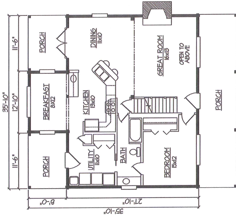
FIRST FLOOR PLAN FIRST FLOOR - 1100 SF TOTAL - 1821 SF
