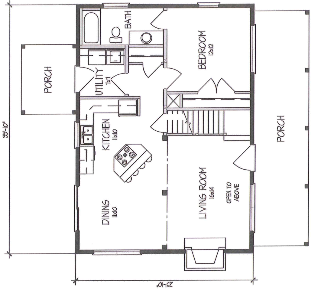
FIRST FLOOR PLAN FIRST FLOOR PLAN - 925 SF TOTAL - 1536 SF
