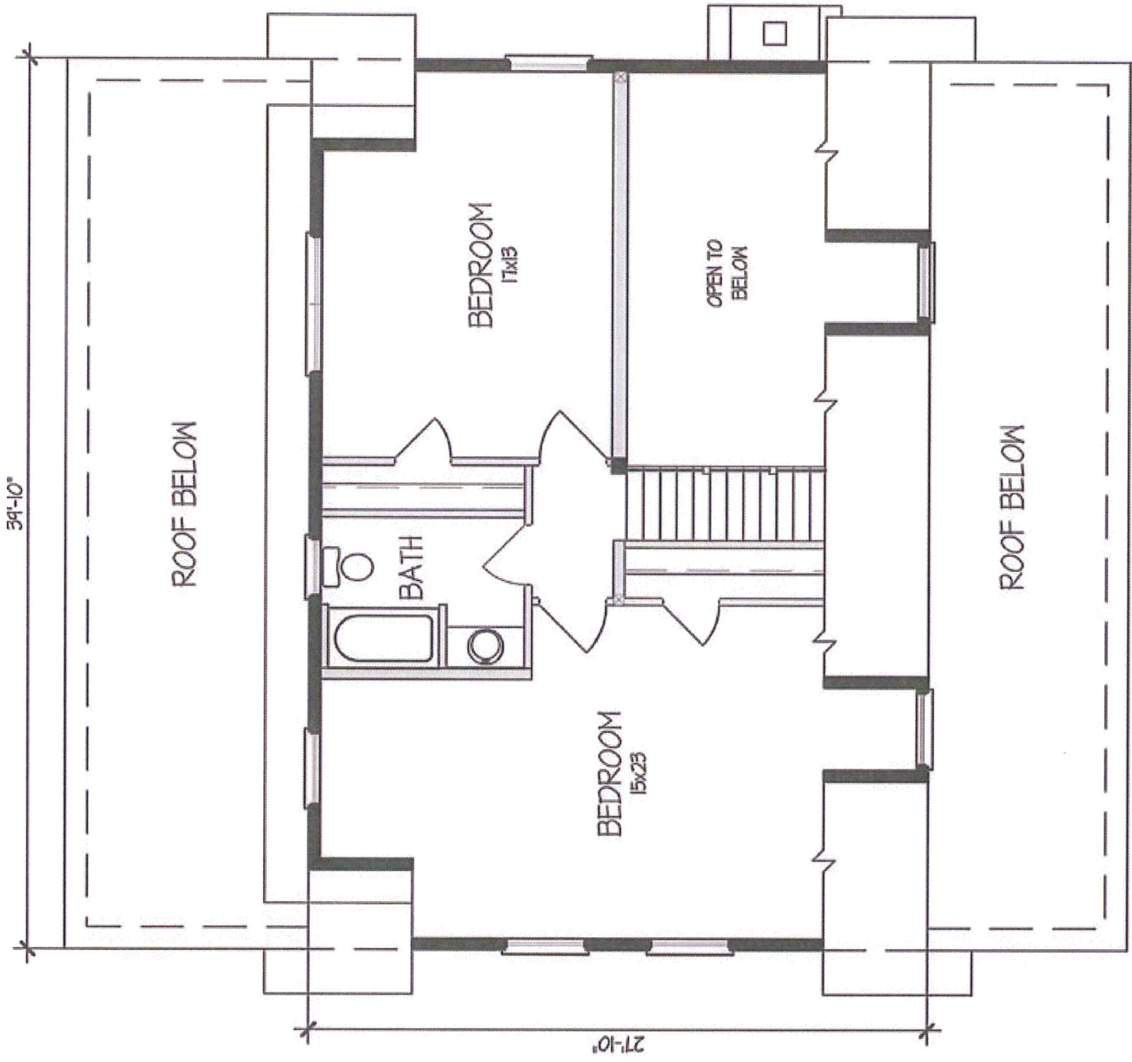
SECOND FLOOR PLAN SECOND FLOOR PLAN - 668 5F
